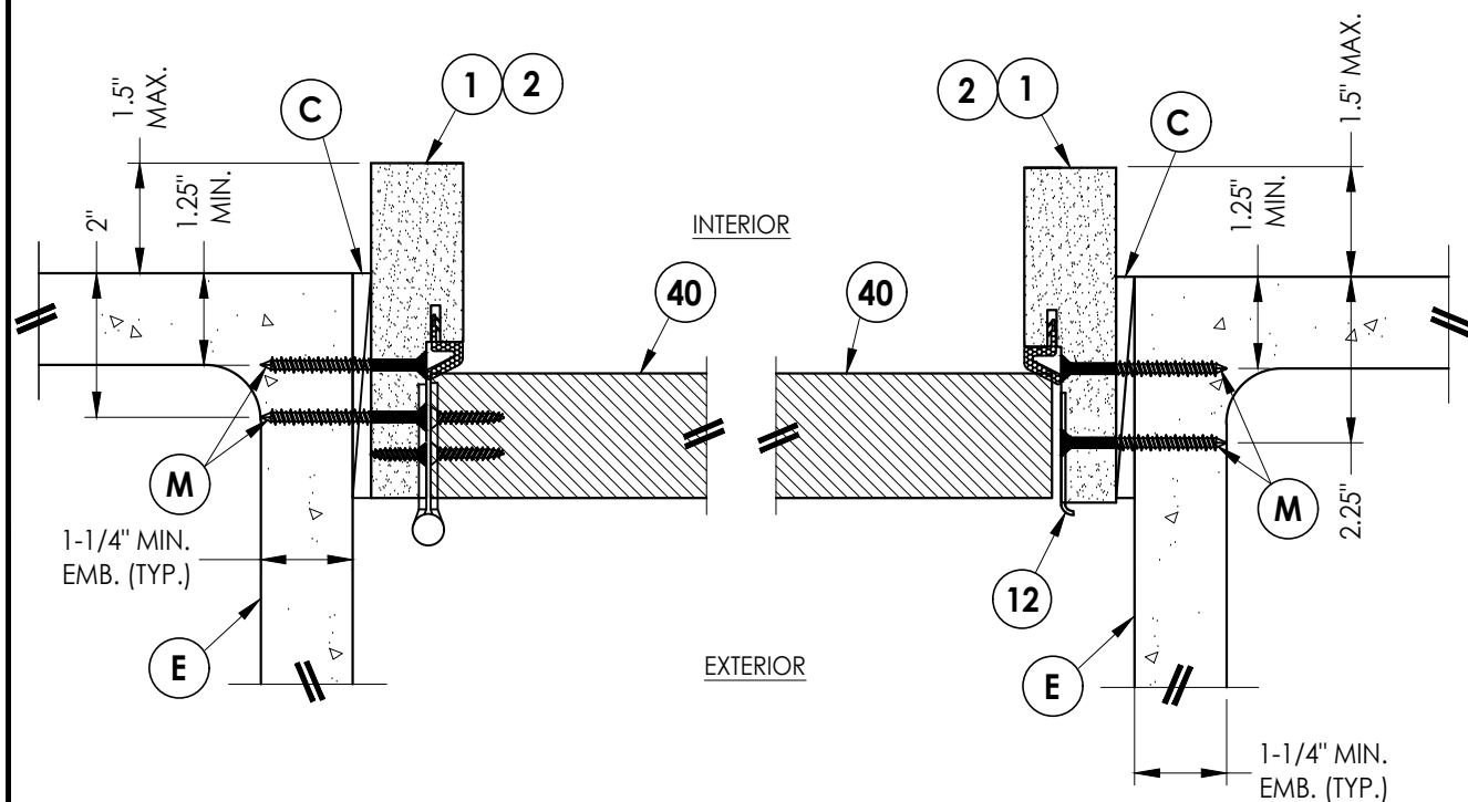
1 HORIZONTAL CROSS SECTION 9 Shown Direct to Masonry Outswing only w/ 4-9/16" jamb Single door only (N/A W/ Sidelites)
