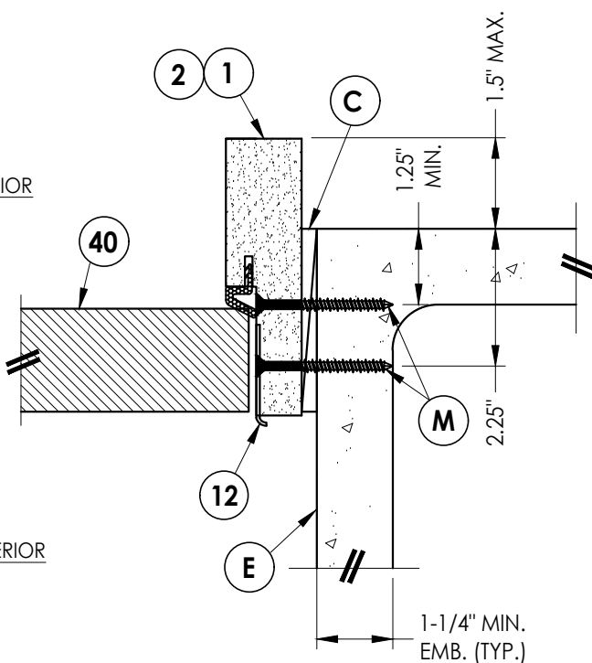
2 9 HORIZONTAL CROSS SECTION Shown Direct to Masonry Outswing only w/ 4-9/16" jamb Single door only (N/A W/ Sidelites)
