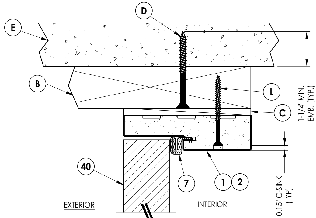
4 5 VERTICAL CROSS SECTION Outswing shown (Inswing similar)
